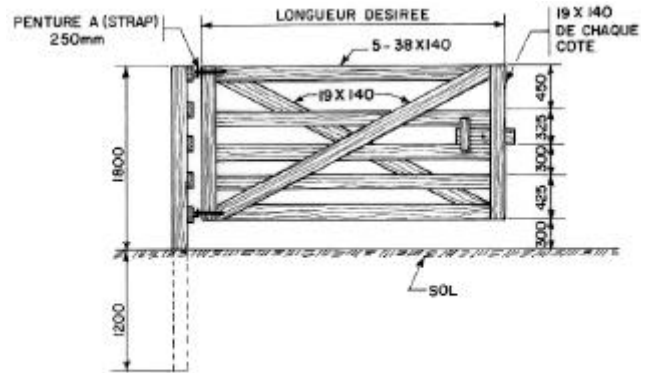
DETAIL DE BARRIERE
