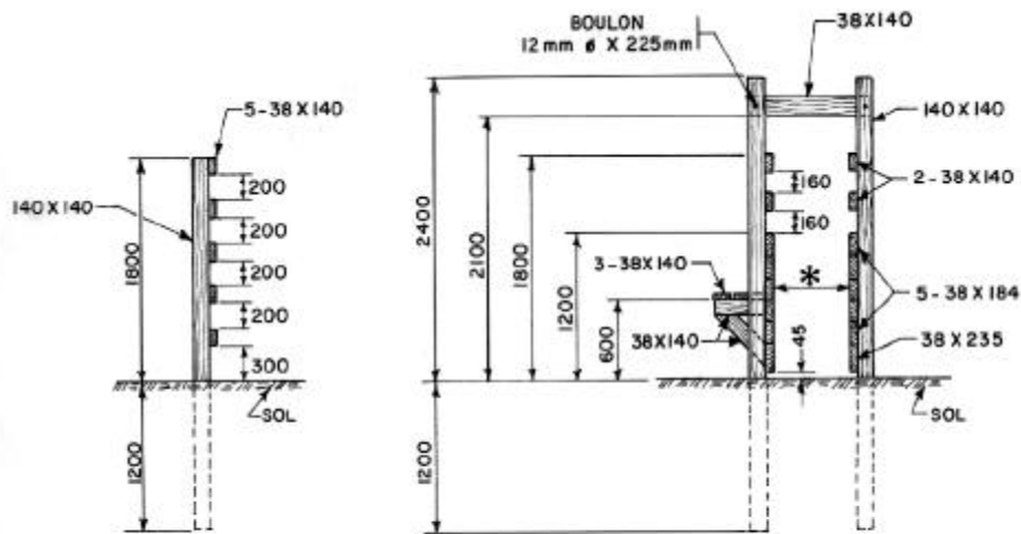
DETAIL DE BARRIERE
