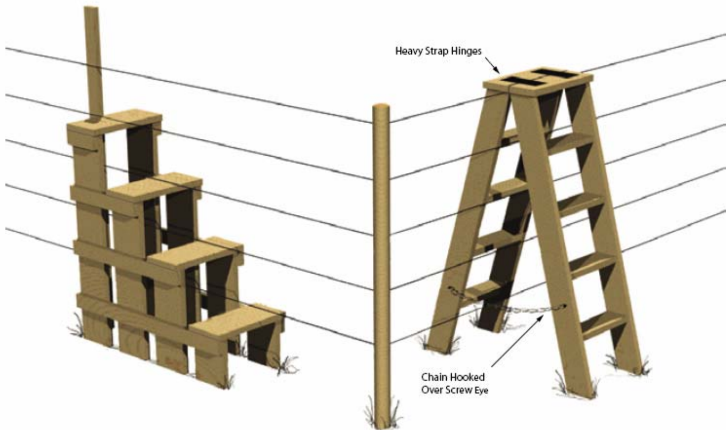
Figure 7. Stile design alternatives.
